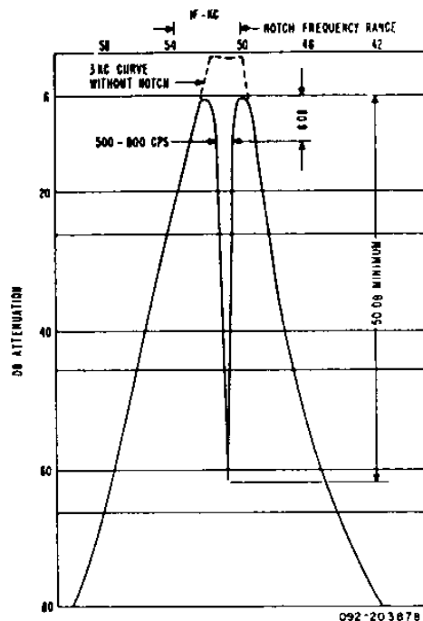
Figure 8. IF Selectivity Curve With Notch
