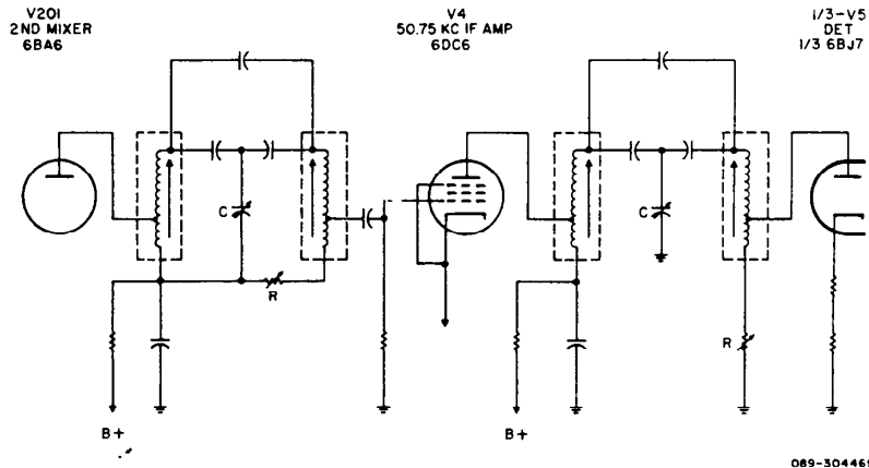
Figure 12. Equivalent Schematic Diagram of 50.75KC IF System
