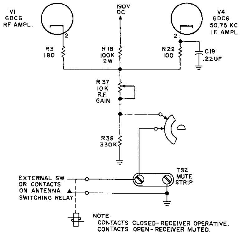
Figure 5. Schematic Diagram of Remote Receive-Standby Circuitry
